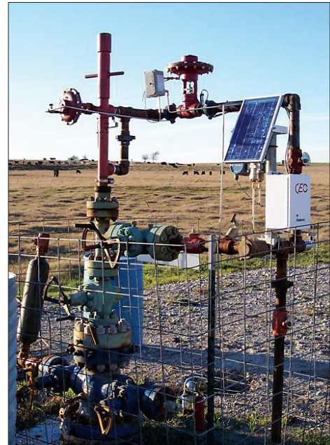
Latching solenoid valve in use on Barnett Shale well with RepidFlo™ plunger and CEO™ Three Plus Controller.
